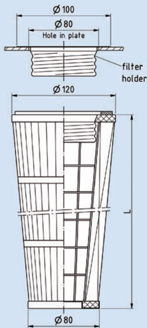
raw gas side installation with Thread Rd 2
