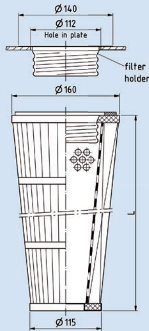
raw gas side installation with Thread Rd 100
