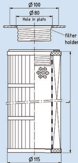
raw gas side installation with Thread Rd 72
