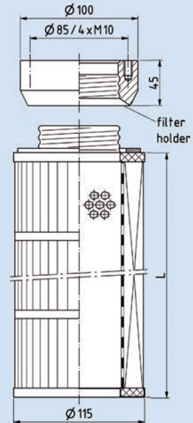
raw gas side installation with Thread Rd 7
